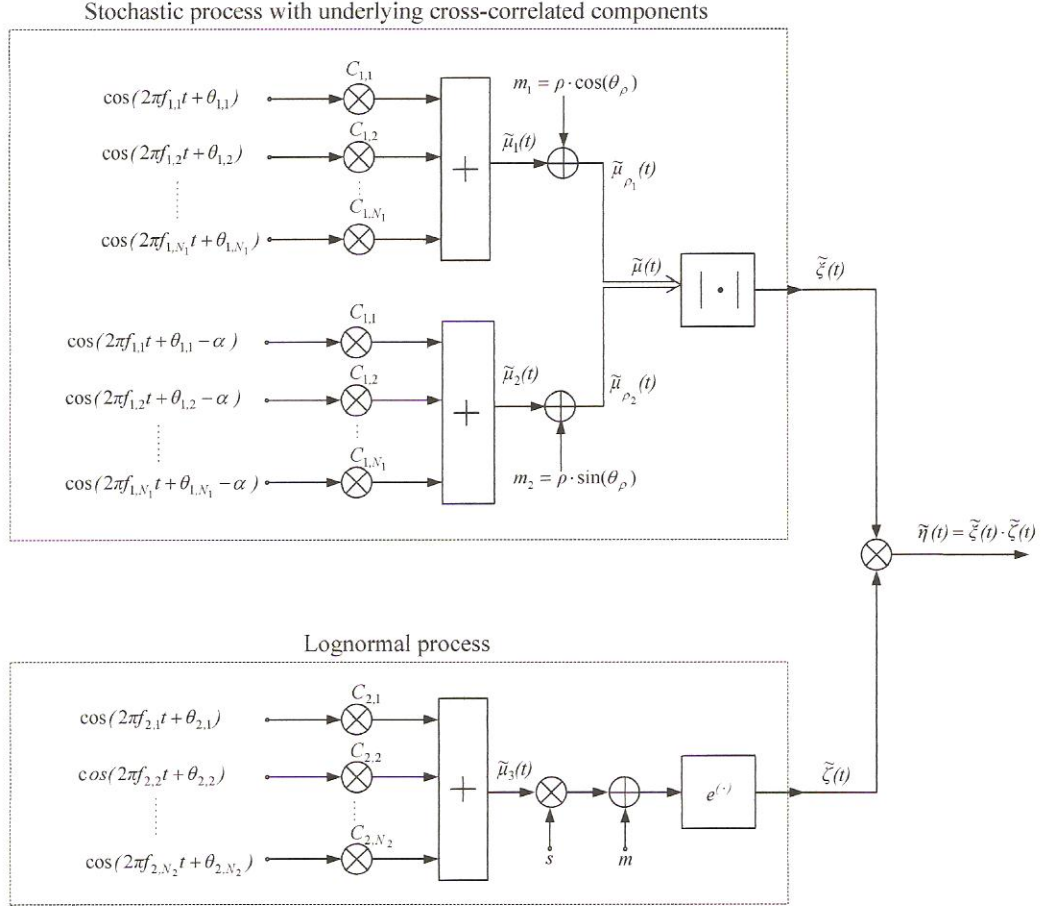
Figure 2 – Structure of the deterministic simulation system
