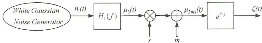
Figure 1 – Analytical model for lognormal process
