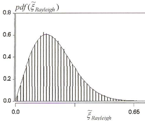
Figure 5 – Histogram versus analytical pdf for \tilde{\xi}(t) Rayleigh distributed ( \alpha = 90^\circ and \rho \rightarrow 0 )
