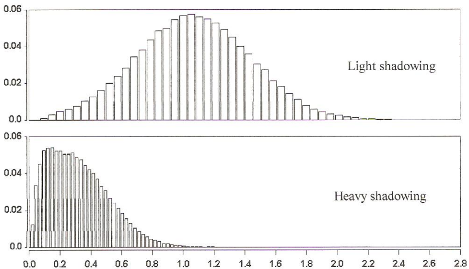
Figure 7 – Histogram of \tilde{\eta} , revealing the signal distribution
