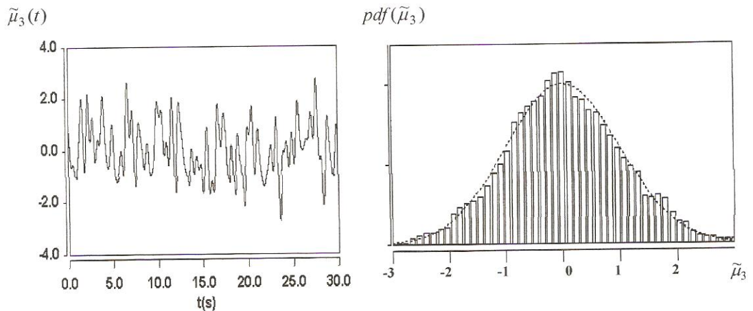
Figure 4 – Simulation of Gaussian noise process \tilde{\mu}_3(t) :
