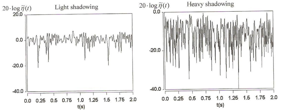
Figure 3 – Simulation of envelope \tilde{\eta}(t)
